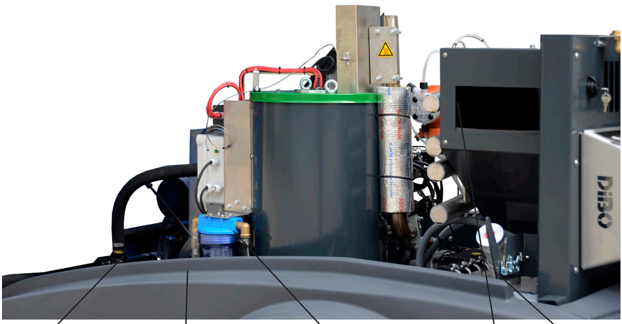
Heat Exchanger Water tank Water filter bilge pump Air Outlet Canal Fuel tank
